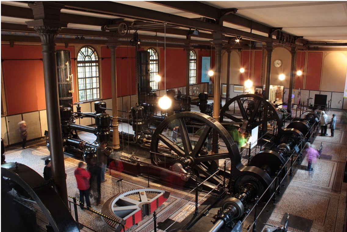
The double-acting piston pumps and air pressure vessels in the Hochablass water pumping station (1879). Photo: Felix Hartmann, via Wikimedia Commons
