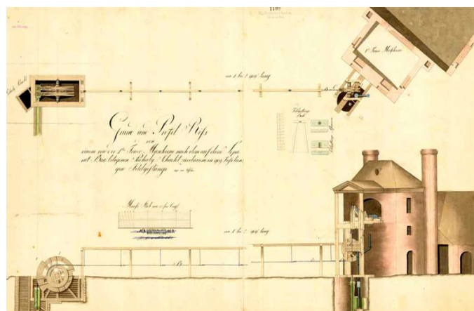
Drawing of the Newcomen Atmospheric Engine, imported from Britain to Friedrich Mine in 1788, the first steam engine on Silesian soil. Samuel Homfray (1762-1822) was its English manufacturer, and subsequently new separate condenser engines pioneered by Boulton & Watt were imported from Britain, to Silesia, copied (there were no patent rights) and manufactured locally to facilitate the construction of a grand and unified adit system to drain the base of the ore-ground, for all time.
